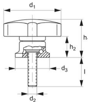
grub screw
