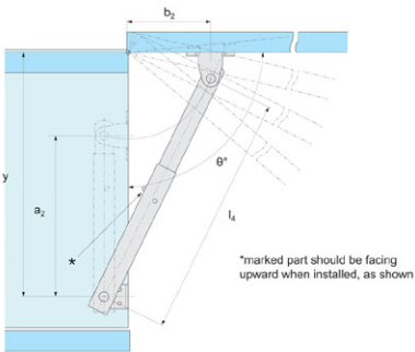
Installation with piano or butt hinge
