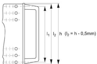
mounting version two
