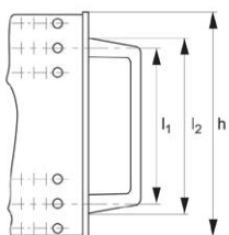
mounting of 19" front panels
