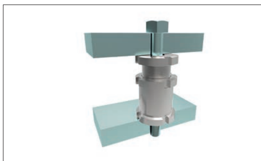
Plunger blocks - even multiple bearings can be levelled easily and precisely, here part no. 62000 is in use.
