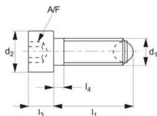
round ball
